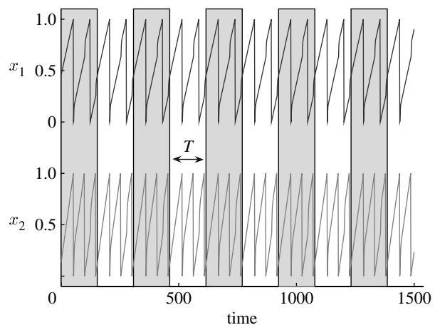
Figure 3. Time series of oscillators 1 and 2 (equations (4.1) and (4.3)) with \varepsilon=8 , \alpha=100 , \tau_1=\tau_2=1 , in a 2 : 3 mode-locked state. The common time frame 'T' is marked with grey and white bands. Note that oscillators x_1 (top graph) fires two spikes for every three spikes of oscillator x_2 (bottom graph) so that oscillator x_1 has a two-cycle attractor while oscillator x_2 has a three-cycle attractor.
